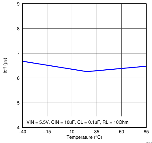
图 5-14. t_{OFF} vs Temperature ( V_{IN} = 5.5\text{ V} )
