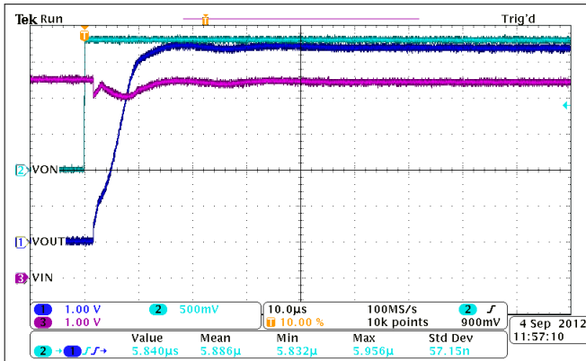
图 5-18. Turn-On Response Time ( V_{IN} = 5.5\text{ V} , C_{IN} = 10\text{ }\mu\text{F} , C_L = 1\text{ }\mu\text{F} , R_L = 10\text{ }\Omega )
