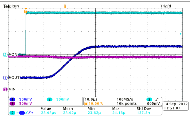
图 5-19. Turn-On Response Time ( V_{IN} = 1.4\text{ V} , C_{IN} = 10\text{ }\mu\text{F} , C_L = 1\text{ }\mu\text{F} , R_L = 10\text{ }\Omega )
