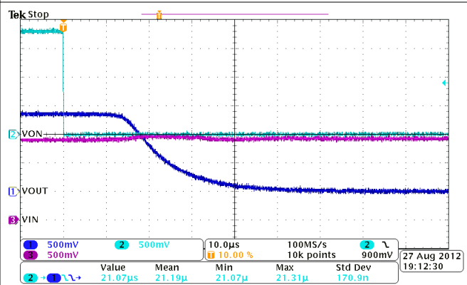
图 5-23. Turn-Off Response Time ( V_{IN} = 1.4\text{ V} , C_{IN} = 10\text{ }\mu\text{F} , C_L = 1\text{ }\mu\text{F} , R_L = 10\text{ }\Omega )
