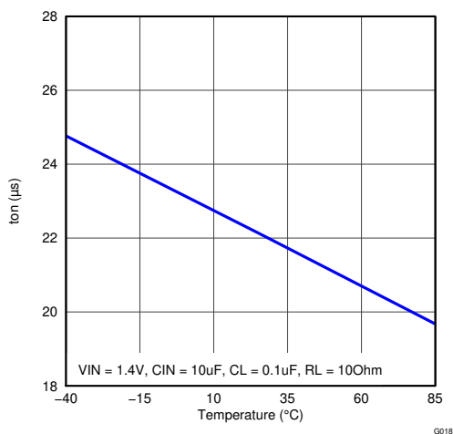
图 5-15. t_{ON} vs Temperature ( V_{IN} = 1.4\text{ V} )
