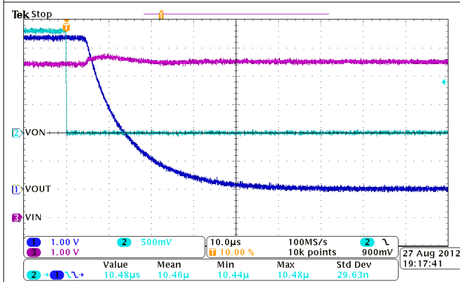
图 5-22. Turn-Off Response Time ( V_{IN} = 5.5\text{ V} , C_{IN} = 10\text{ }\mu\text{F} , C_L = 1\text{ }\mu\text{F} , R_L = 10\text{ }\Omega )
