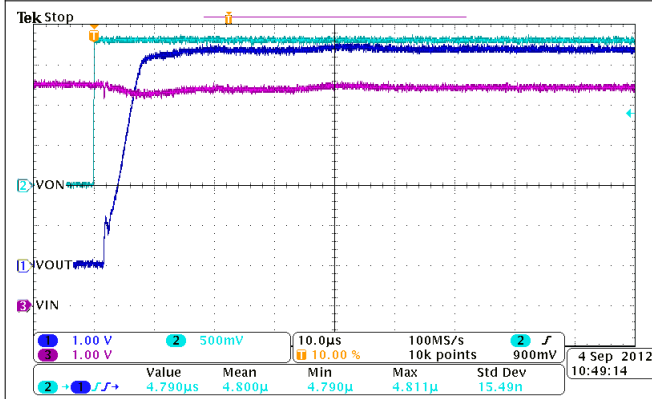
图 5-20. Turn-On Response Time ( V_{IN} = 5.5\text{ V} , C_{IN} = 10\text{ }\mu\text{F} , C_L = 0.1\text{ }\mu\text{F} , R_L = 10\text{ }\Omega )
