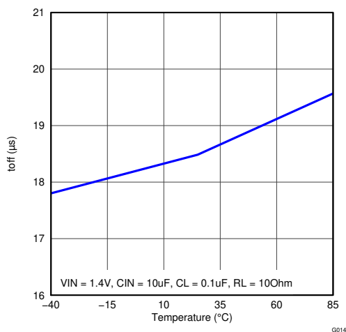
图 5-16. t_{OFF} vs Temperature ( V_{IN} = 1.4\text{ V} )
