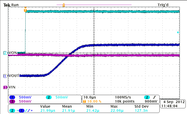
图 5-21. Turn-On Response Time ( V_{IN} = 1.4\text{ V} , C_{IN} = 10\text{ }\mu\text{F} , C_L = 0.1\text{ }\mu\text{F} , R_L = 10\text{ }\Omega )
