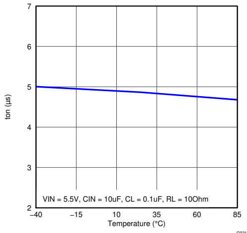
图 5-13. t_{ON} vs Temperature ( V_{IN} = 5.5\text{ V} )
