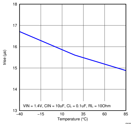
图 5-11. t_R vs Temperature ( V_{IN} = 1.4 V)
