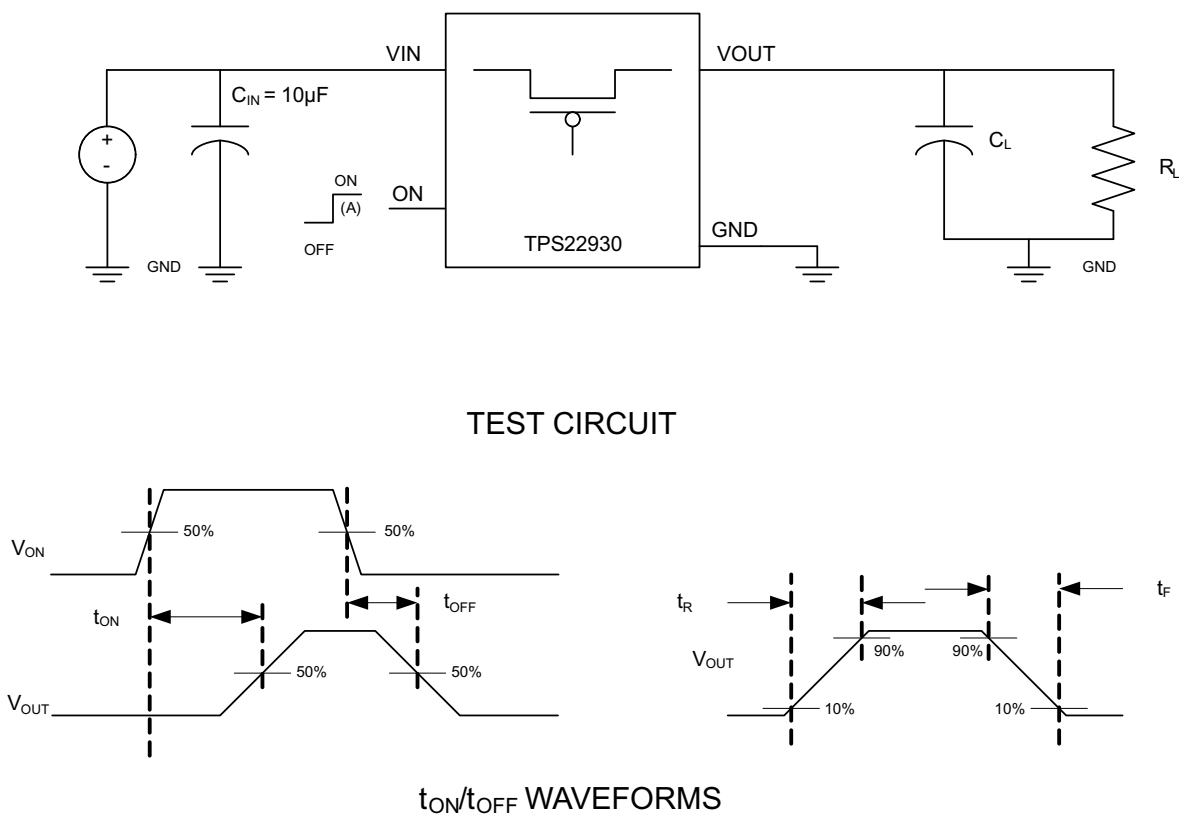
图 7-1. Test Circuit and t ON /t OFF Waveforms
