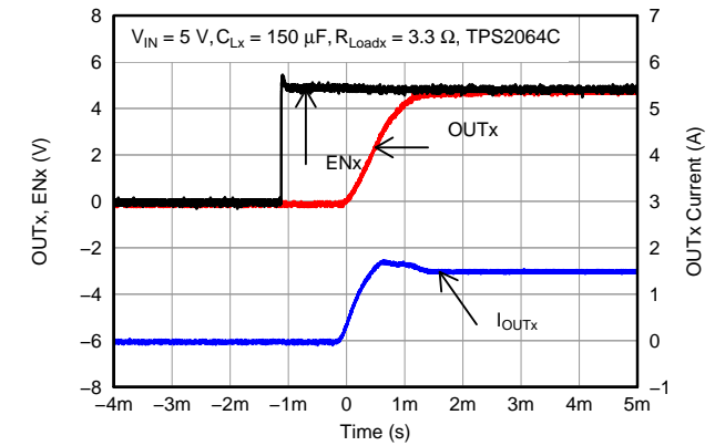
Figure 24. TPS2064C Enable into 3.3 Ω and 150-µF Load
