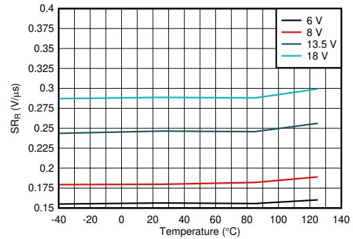
图 7-8. V_{OUT} Slew Rate Rising ( SR_R ) vs Temperature
