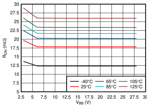
I_{OUT} = 200\text{ mA} V_{EN} = 5\text{ V} V_{DIAG\_EN} = 0\text{ V} R_{SNS} = 1\text{ k}\Omega V_{BB} = 13.5\text{ V} 图 7-5. On Resistance ( R_{ON} ) vs V_{BB}
