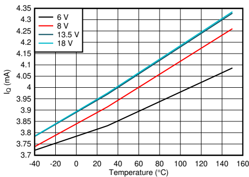
I_{OUT} = 0\text{ A} V_{EN} = 5\text{ V} V_{DIAG\_EN} = 5\text{ V} R_{SNS} = 1\text{ k}\Omega V_{SEL1} = 0\text{ V} 图 7-3. Quiescent Current ( I_Q ) vs Temperature
