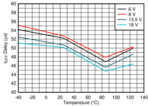
图 7-7. Turn-off Delay Time ( t_{DF} ) vs Temperature
