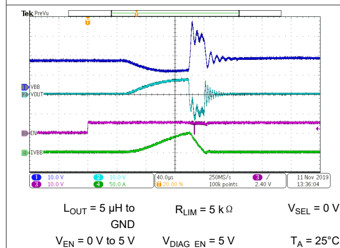
图 7-27. Device Version B Short Circuit Event
