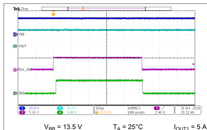
图 7-25. SNS Output Current Measurement Enable on DIAG_EN PWM
