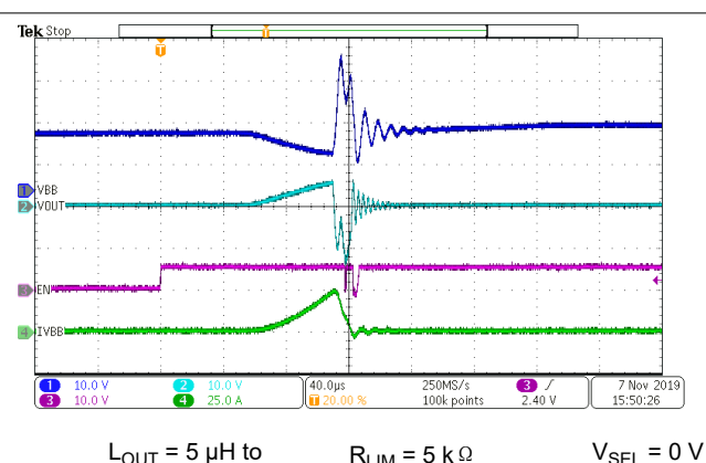
图 7-26. Device Version A Short Circuit Event
