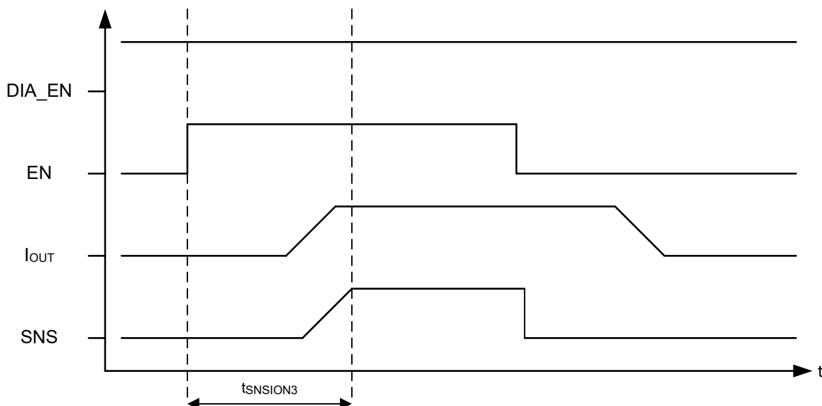
图 9-11. Current Sensing in Low-Duty Cycle Applications
