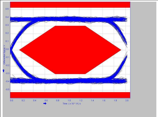
Figure 34. Eye-Diagram With EVM, Without TPD3S0x4
