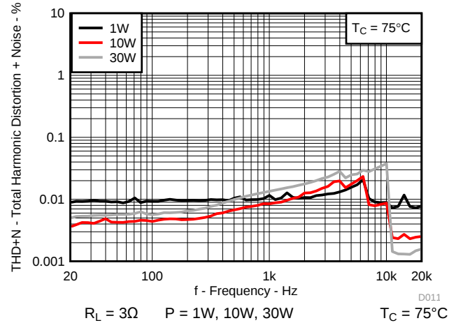
Figure 11. Total Harmonic Distortion+Noise vs Frequency
