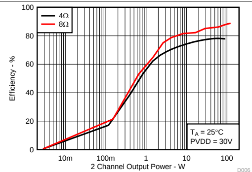
Figure 6. System Efficiency vs Output Power, AD-mode
