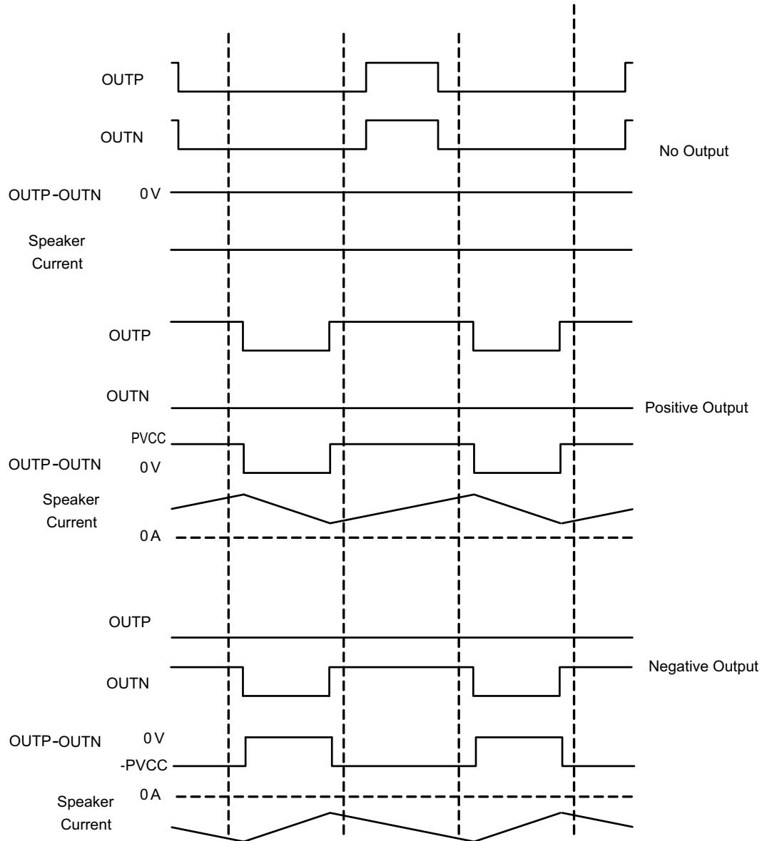
图 7-3. Low-Idle-Current 1SPW Modulation
