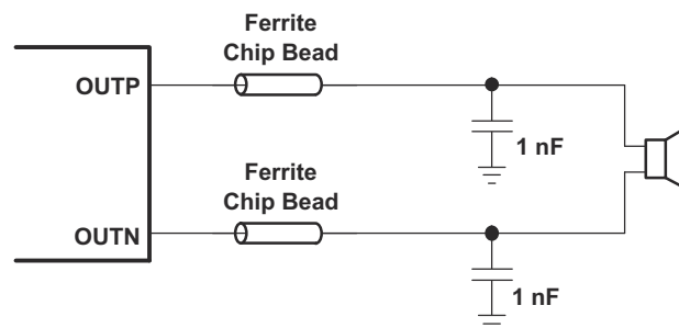
图 8-3. Typical Ferrite Chip Bead Filter (Chip Bead Example: NFZ2MSM series from Murata)
