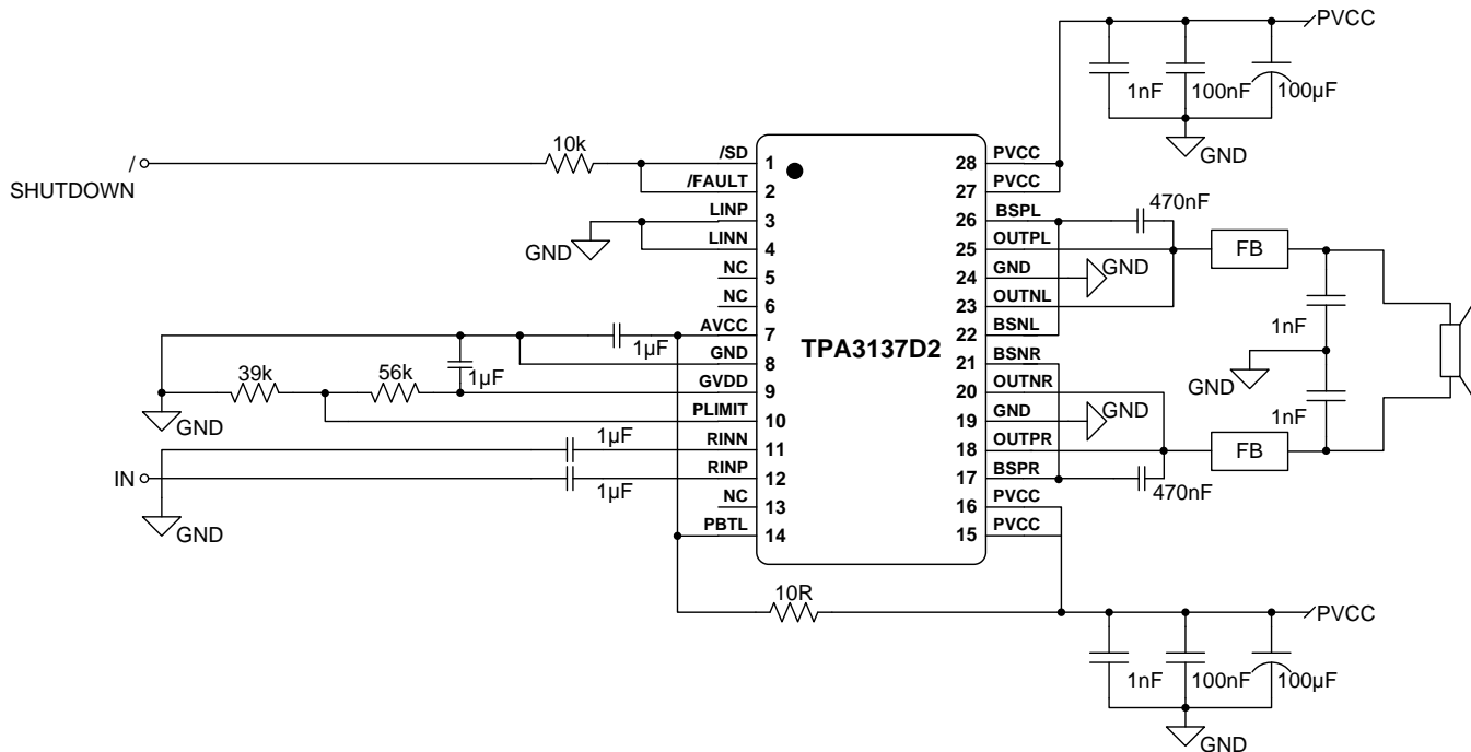
Figure 19. Stereo Class-D Amplifier with PBTTL Output and Single-Ended Input with Spread Spectrum Modulation
