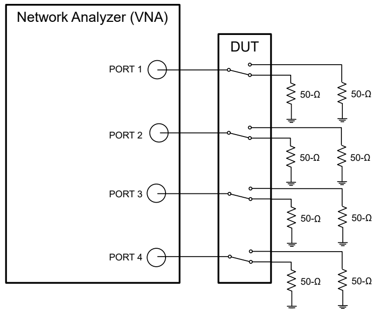
图 6-4. 串扰 (Xtalk)
