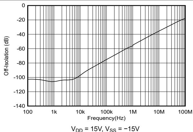
图 5-22. Off-Isolation vs Frequency
