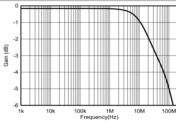
图 5-24. On Response vs Frequency
