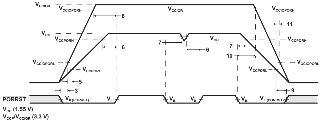
Figure 5-1. \overline{PORRST} Timing Diagram
