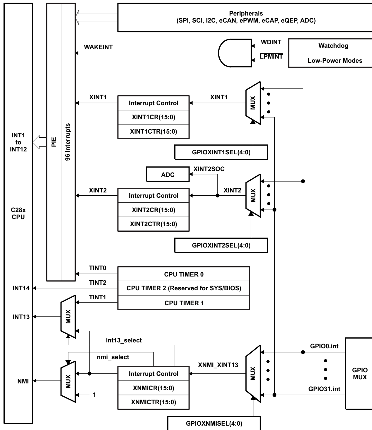
Figure 6-23. External and PIE Interrupt Sources
