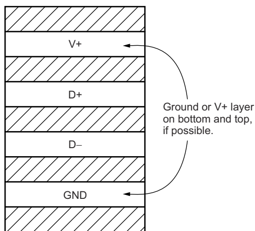
Figure 9-4. Suggested PCB Layer Cross-Section
