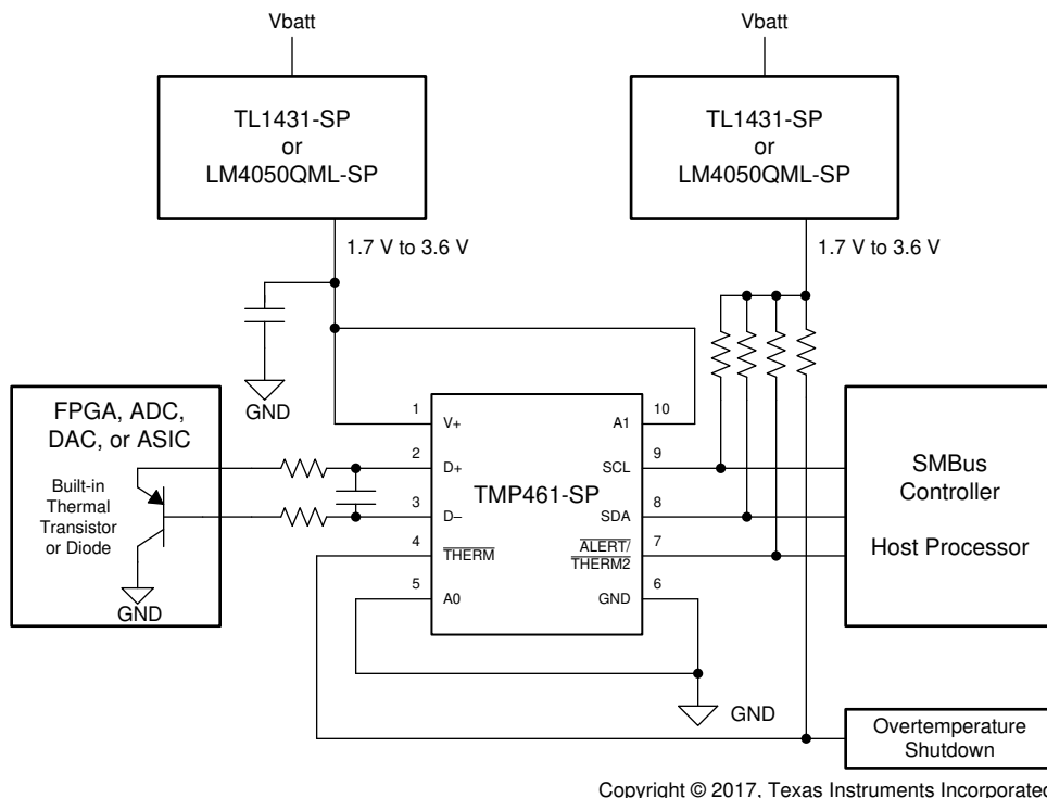
图 18. TMP461-SP Basic Connections Using a Processor Built-In Remote Transistor
