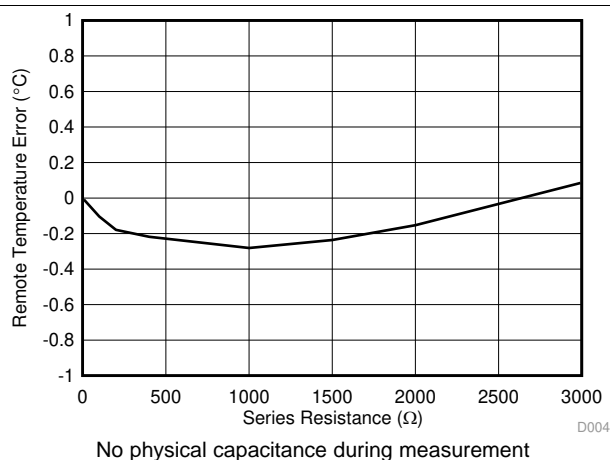
图 5. Remote Temperature Error vs Series Resistance
