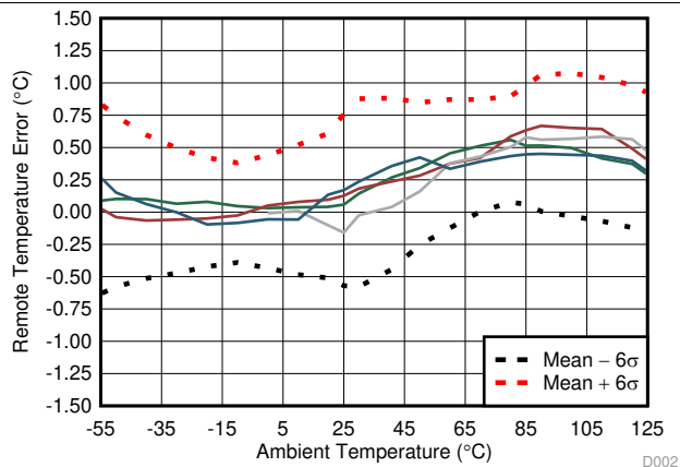
图 3. Remote Temperature Error vs Ambient Temperature
