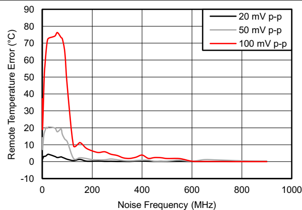
图 6-7. Remote Temperature Error vs. Remote Channel Noise Frequency
