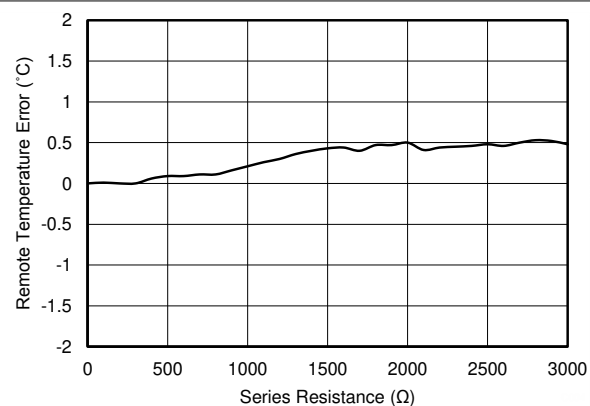
图 6-5. Remote Temperature Error vs. Series Resistance
