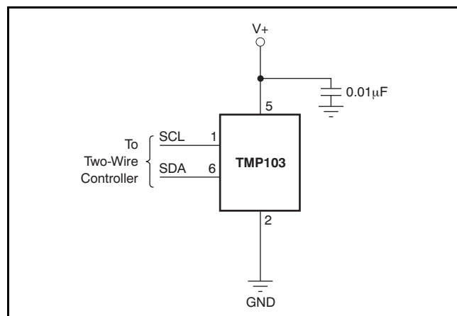
Figure 6. Typical Connections
