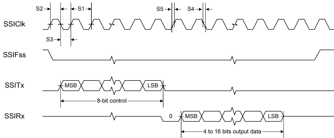
图 23-20. SSI Timing for MICROWIRE Frame Format (FRF=10), Single Transfer
