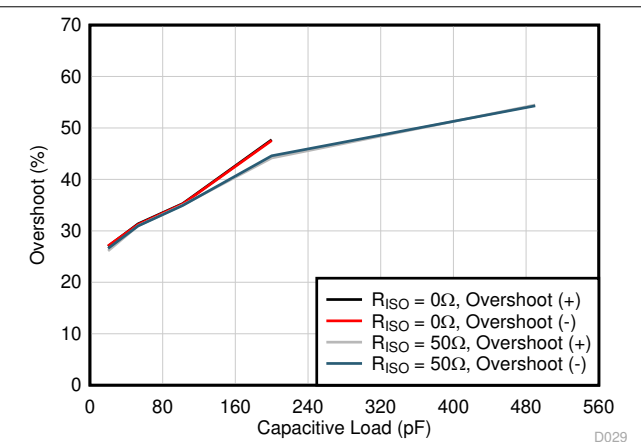
图 6-4. Small-Signal Overshoot vs Capacitive Load (20mV pp Output Step, G = -1 )
