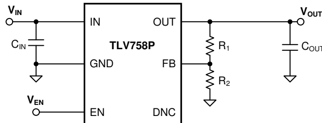
图 7-1. Adjustable Operation
