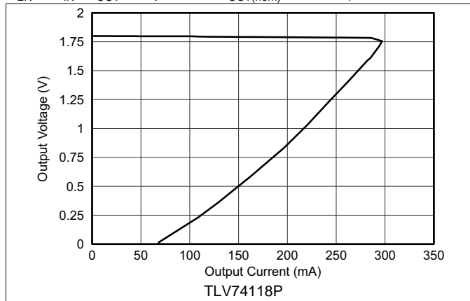
图 19. 1.8-V Output Voltage vs Output Current (Foldback Current Limit)
