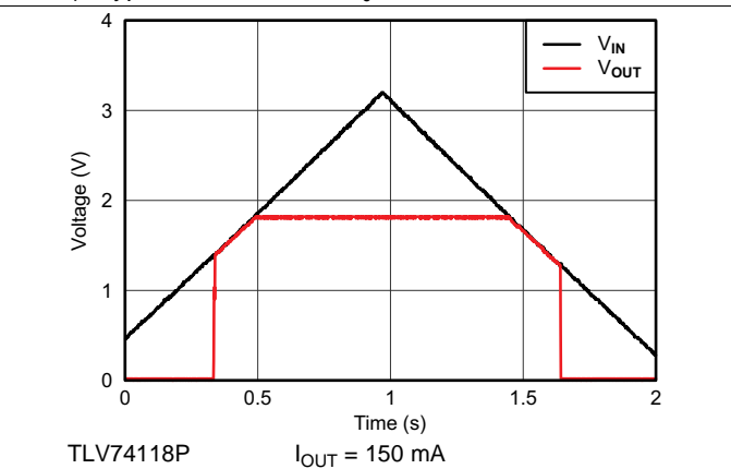
图 20. V_{IN} Power-Up and Power-Down
