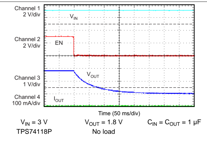
图 22. Shutdown Response With Enable
