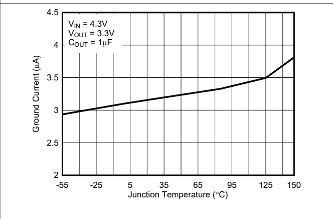
图 6-12. Ground Current vs Junction Temperature for New Chip
