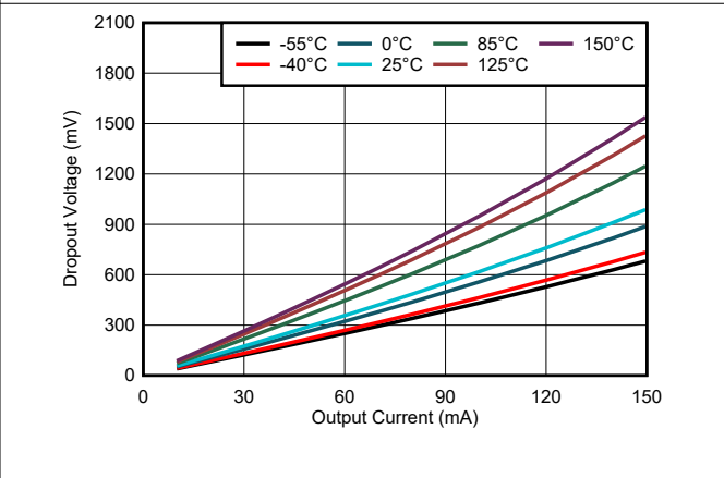
图 6-10. Dropout Voltage vs Output Current for New Chip
