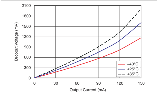
图 6-9. Dropout Voltage vs Output Current for Legacy Chip
