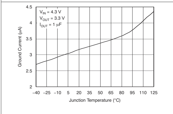
图 6-11. Ground Current vs Junction Temperature for Legacy Chip
