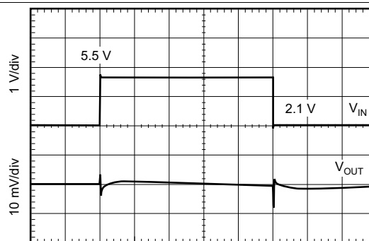
1 ms/div V_{OUT} = 1.8\text{ V} , I_{OUT} = 300\text{ mA} , slew rate = 1\text{ V}/\mu\text{s}
