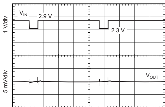
1 ms/div V_{OUT} = 1.8\text{ V} , I_{OUT} = 1\text{ mA} , slew rate = 1\text{ V}/\mu\text{s}
