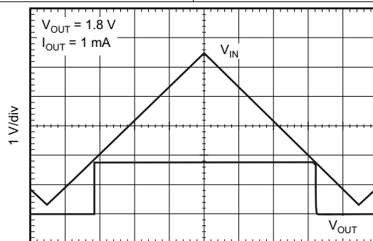
200 ms/div V_{OUT} = 1.8\text{ V} , I_{OUT} = 1\text{ mA}
