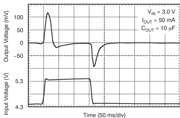
图 8-3. Line Transient Response for Legacy Chip
