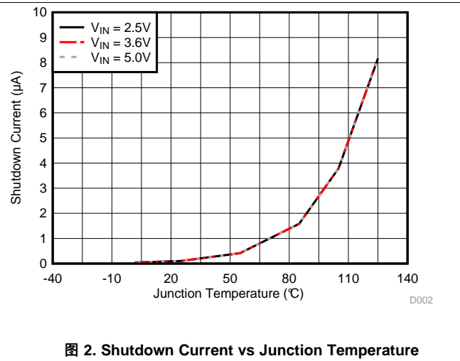
图 2. Shutdown Current vs Junction Temperature
