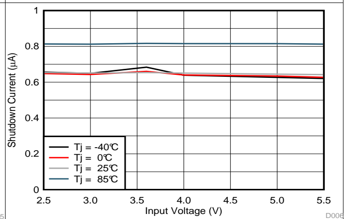
图 4. Shutdown Current
