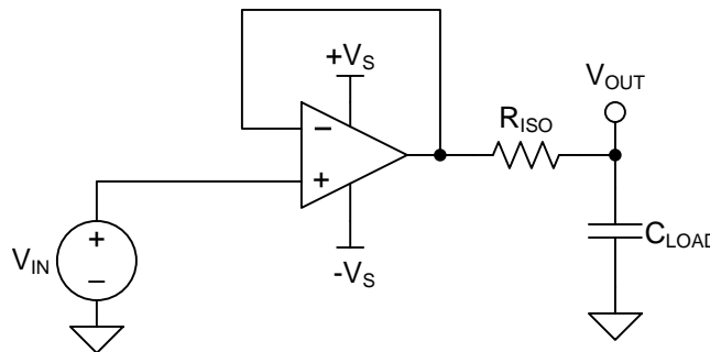
图 29. Unity-Gain Buffer With R_{\text{ISO}} Stability Compensation
