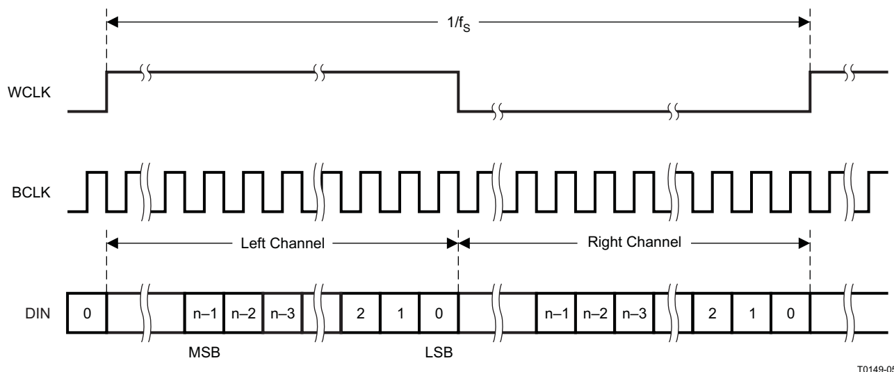
Figure 5-24. Timing Diagram for Right-Justified Mode
