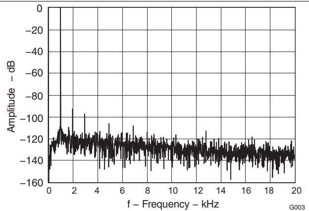
图 6. DAC to Line Output FFT Plot
