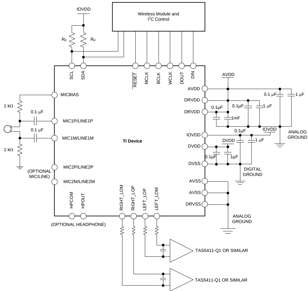
188. Typical Connections for Emergency Call System (E-Call)
