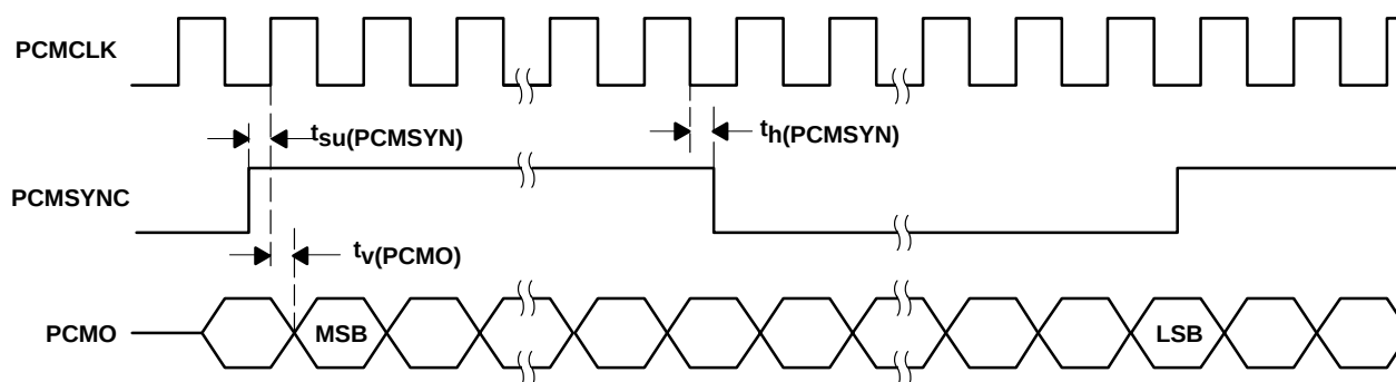
Figure 5. Transmit Timing Diagram, 128 kHz
