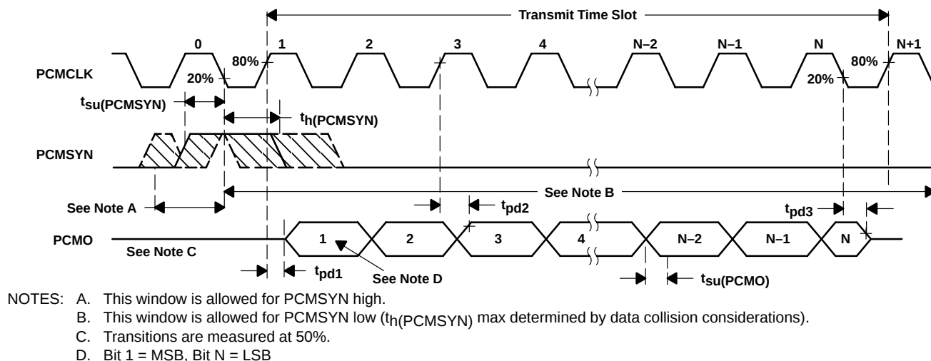
Figure 1. Transmit Timing Diagram (2.048 MHz)
