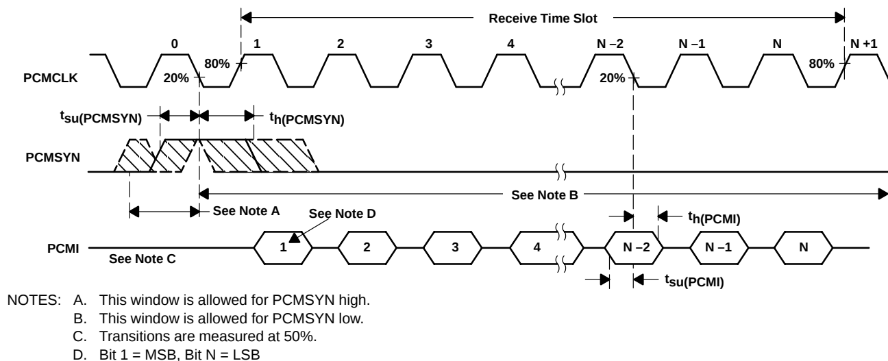
Figure 2. Receive Timing Diagram (2.048 MHz)
