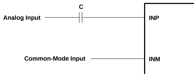
Figure 2–18. Single-Ended Input
