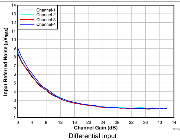
图 13. Input-Referred Noise vs Channel Gain
