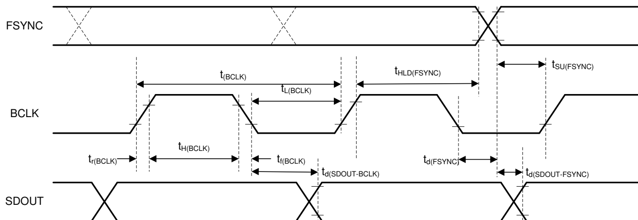
图 7-2. TDM (With BCLK_POL = 1), I 2 S, and LJ Interface Timing Diagram
