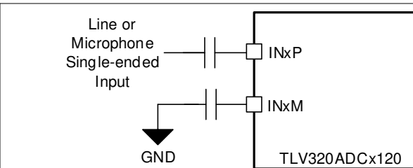
图 8-15. Single-Ended, AC-Coupled Input Connection
