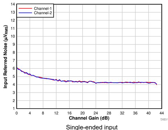
图 7-10. Input-Referred Noise vs Channel Gain
