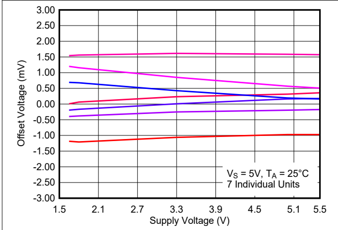
图 6-50. Offset Voltage vs. Supply Voltage, 25°C
