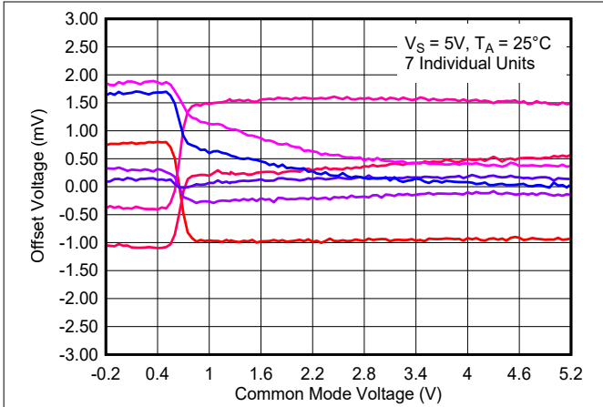
图 6-48. Offset Voltage vs. Common Mode Voltage, 5 V
