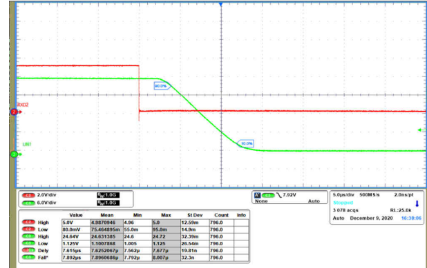
图 10-3. Recessive to Dominant Propagation
