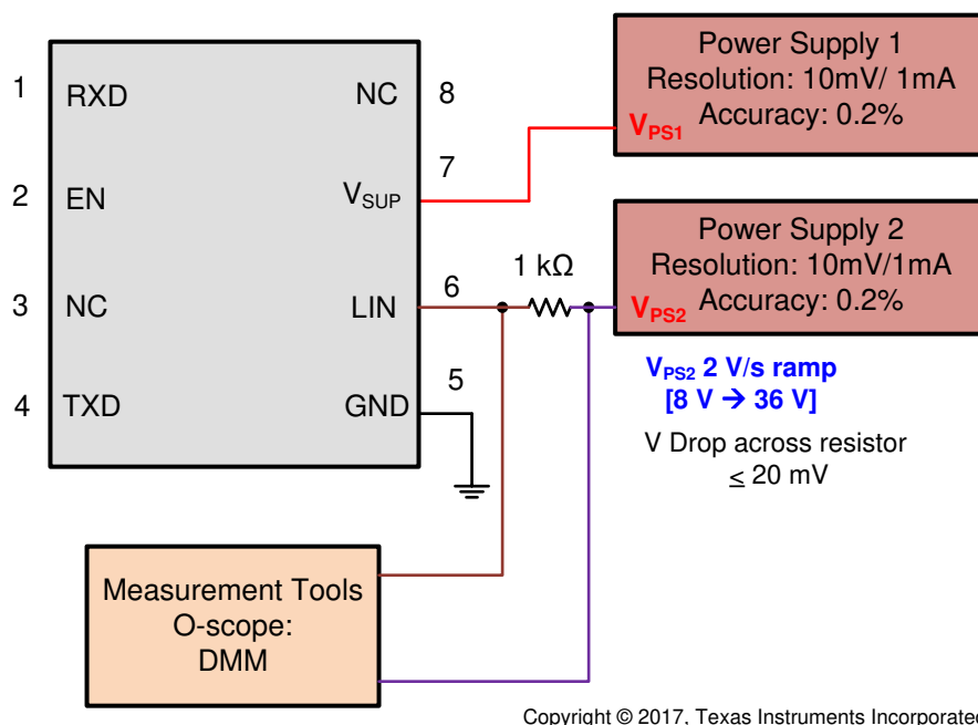
图 8-8. Test Circuit for I_{BUS\_PAS\_rec} Param 14
