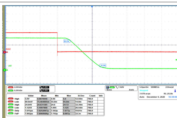
图 10-3. Recessive to Dominant Propagation
