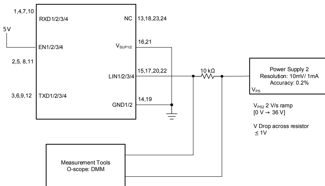
图 8-9. Test Circuit for I_{BUS} NO BAT Loss of Battery
