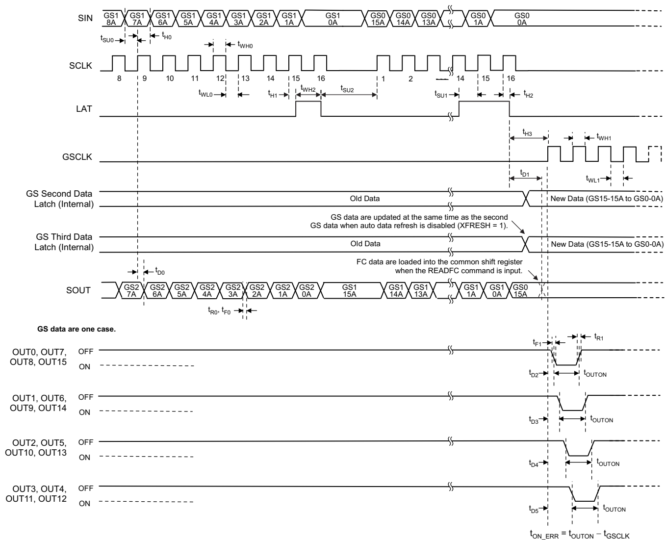
Figure 10. Timing Diagram
