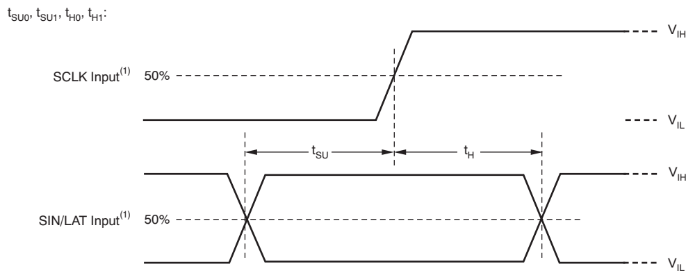
Figure 4. Input Timing
