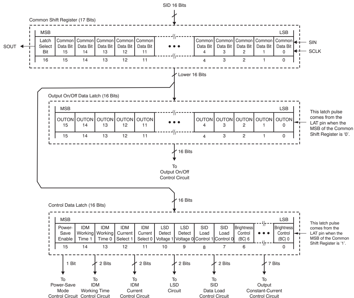
Figure 20. Common Shift Register and Control Data Latches Configuration
