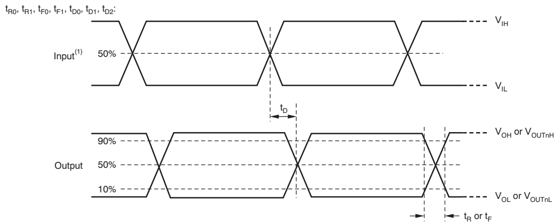
Figure 5. Output Timing
