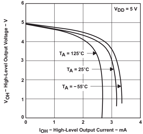
图 6-14. High-Level Output Voltage vs High-Level Output Current
