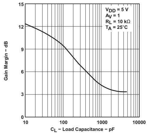
图 6-58. Gain Margin vs Load Capacitance
