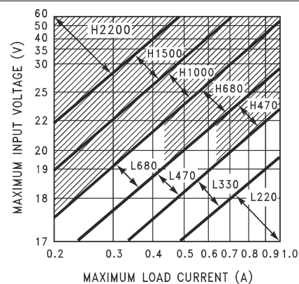
Figure 9-5. TL2575-15
