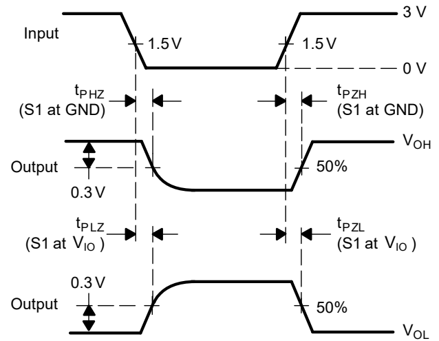
VOLTAGE WAVEFORMS
