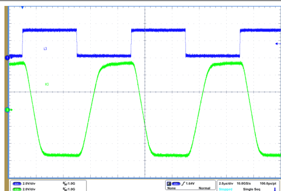
V_{CC} = 3.3V 总线负载 = 5k\Omega || 2.5nF 250kbps SLR = V_{IO}
