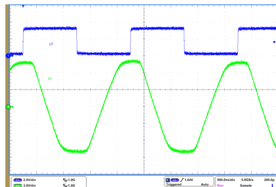
V_{CC} = 5V 总线负载 = 5k\Omega || 1nF 1Mbps SLR = GND
