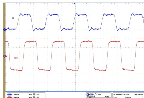
V_{CC} = 5V 总线负载 = 54\Omega || 50pF SLR = GND 20Mbps 时的方波
