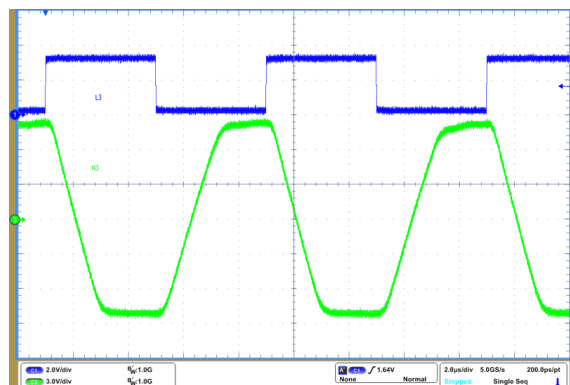
V_{CC} = 5V 总线负载 = 5k\Omega || 2.5nF 250kbps SLR = V_{IO}
