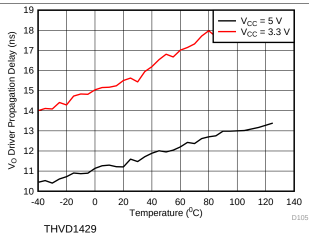
图 5. Driver Propagation Delay vs Temperature
