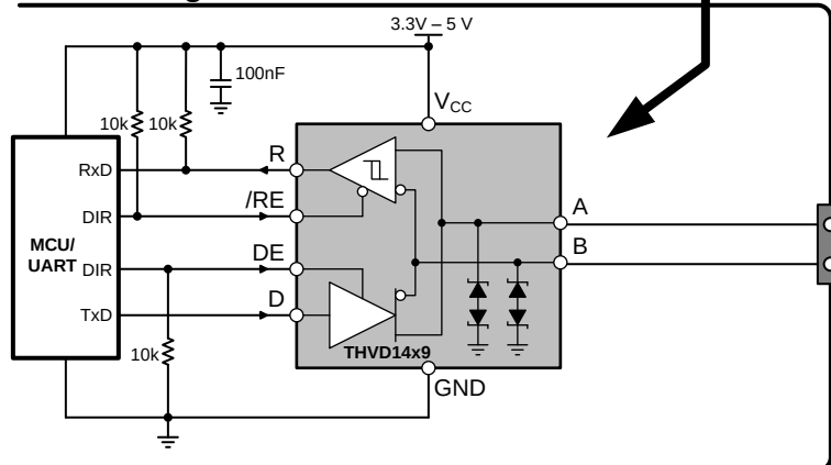
图 25. Implementation of System-Level Surge Protection Using THVD14x9
