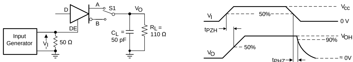
图 13. Measurement of Driver Enable and Disable Times With Active High Output and Pull-Down Load
