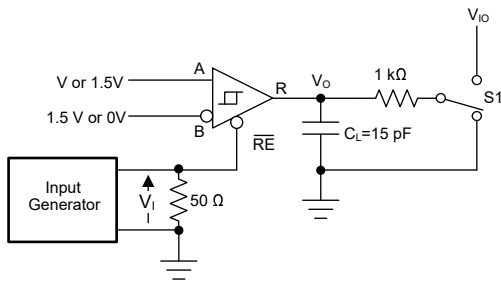
图 6-8. Measurement of Receiver Enable Times With Driver Disabled
