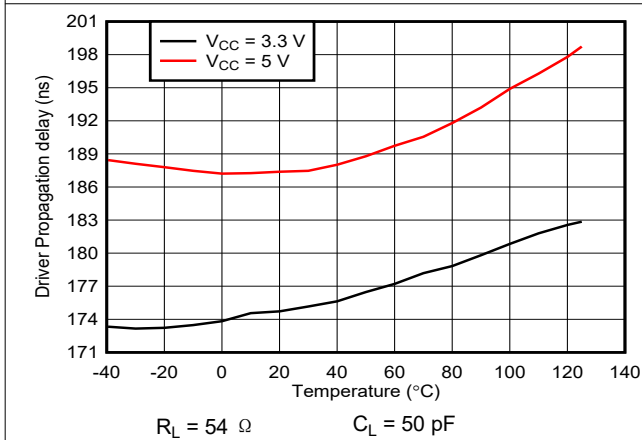
图 5-5. Driver Propagation Delay vs Temperature (500 kbps)
