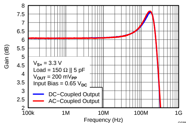
Figure 44. HD BYPASS SMALL-SIGNAL GAIN vs FREQUENCY
