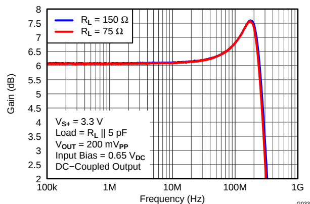
Figure 40. HD BYPASS SMALL-SIGNAL GAIN vs FREQUENCY
