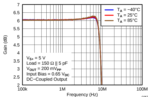
Figure 67. SD SMALL-SIGNAL GAIN vs FREQUENCY
