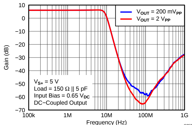
Figure 62. SD LARGE-SIGNAL GAIN vs FREQUENCY
