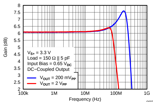
Figure 42. HD BYPASS LARGE-SIGNAL GAIN vs FREQUENCY
