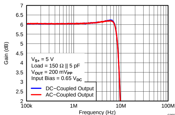
Figure 65. SD SMALL-SIGNAL GAIN vs FREQUENCY
