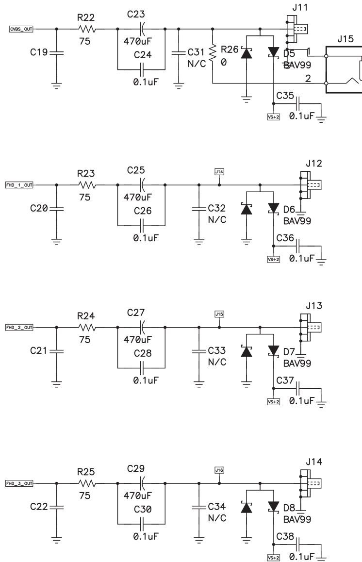
Figure 91. THS7372EVM Schematic 2
