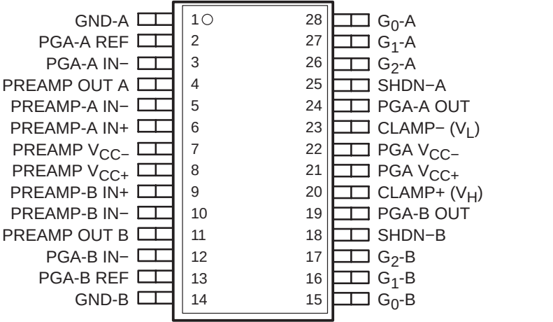
THS7002 PWP PACKAGE (TOP VIEW)
