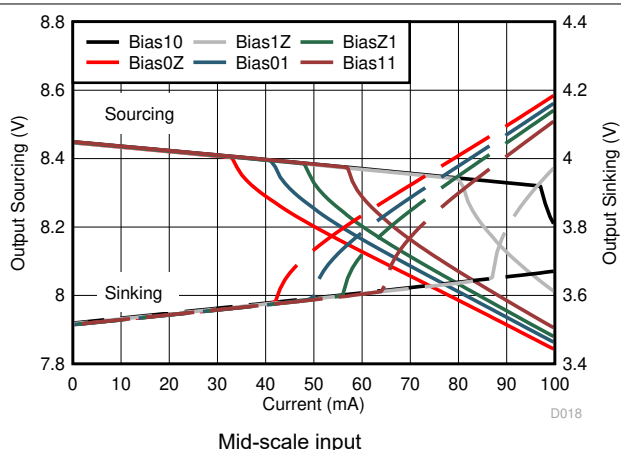
图 6-18. Output Voltage vs Current
