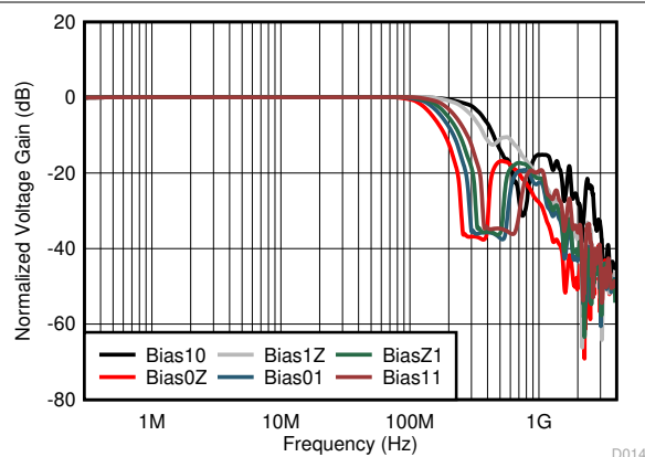
图 6-14. Normalized Large-Signal Frequency Response
