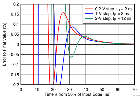
图 6-27. Small- and Large-Signal Step Response
