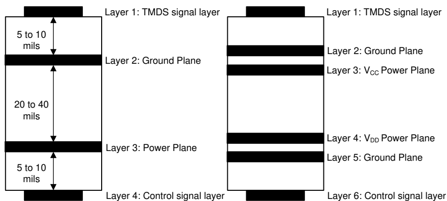
图 9-11. Recommended 4 or 6-Layer PCB Stack
